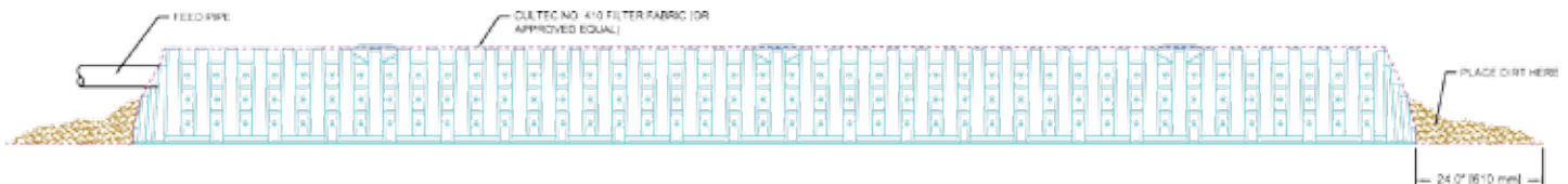
Filter Fabric Installation Profile View
