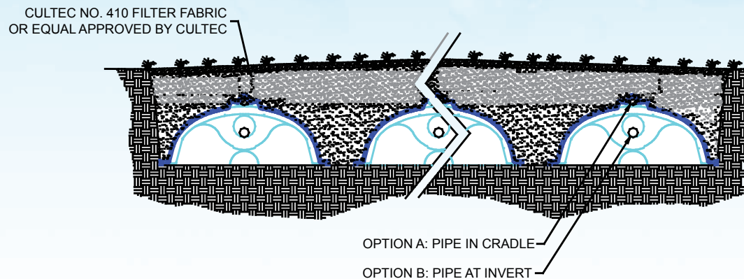
CULTEC Pressure Distribution Options
